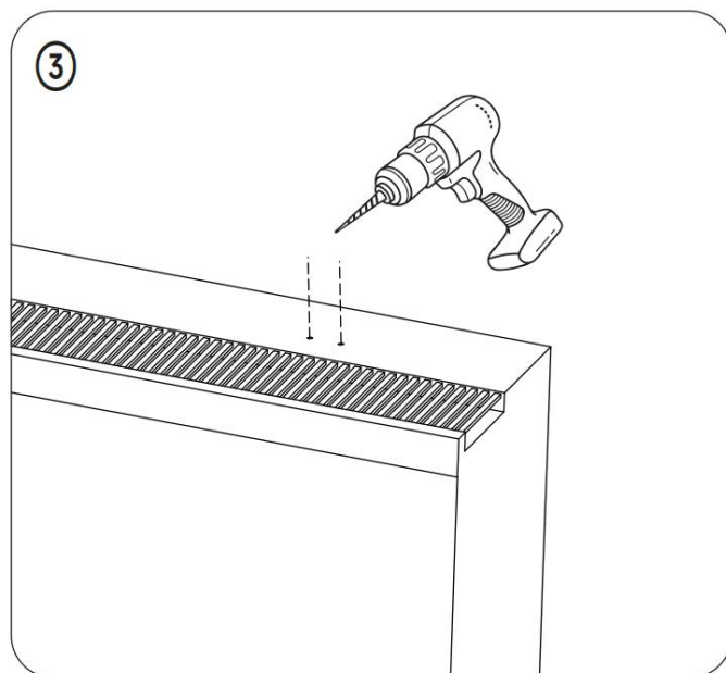
③ Drill the holes according to the installation holes, the recommended drill diameter is 8mm and the hole depth is 45mm. Take care to avoid electrical wires, gas pipes and water pipes to avoid
